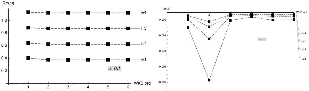
Fig. 2. The real and imaginary part of QNMs with sixth-, fifth-, fourth-, third-, and second-order WKB formula and the eikonal approximation for a=0.1 , M=1 and s=0 mode with the multipole numbers l=(1,2,3,4) .
