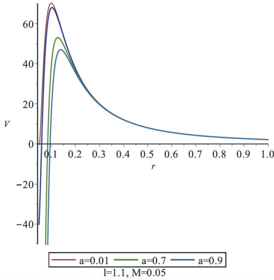
Fig. 1. (color online) V vs. r for massless particles.
