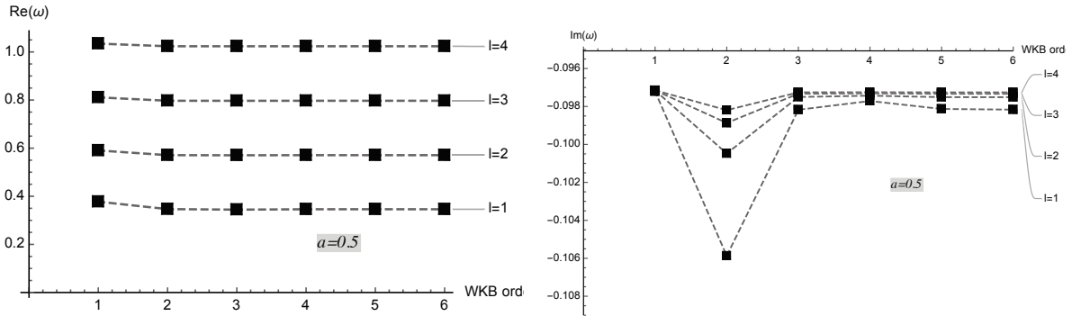
Fig. 3. The real and imaginary part of QNMs with sixth-, fifth-, fourth-, third-, and second-order WKB formula and the eikonal approximation for a=0.5 , M=1 and s=0 mode with the multipole numbers l=(1,2,3,4) .
