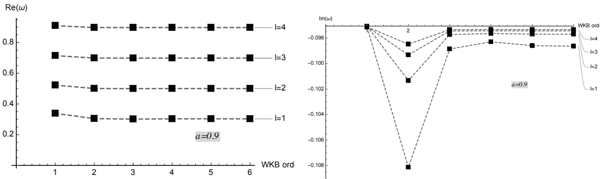
Fig. 4. The real and imaginary part of QNMs with sixth-, fifth-, fourth-, third-, and second-order WKB formula and the eikonal approximation for a=0.9 , M=1 and s=0 mode with the multipole numbers l=(1,2,3,4) .
