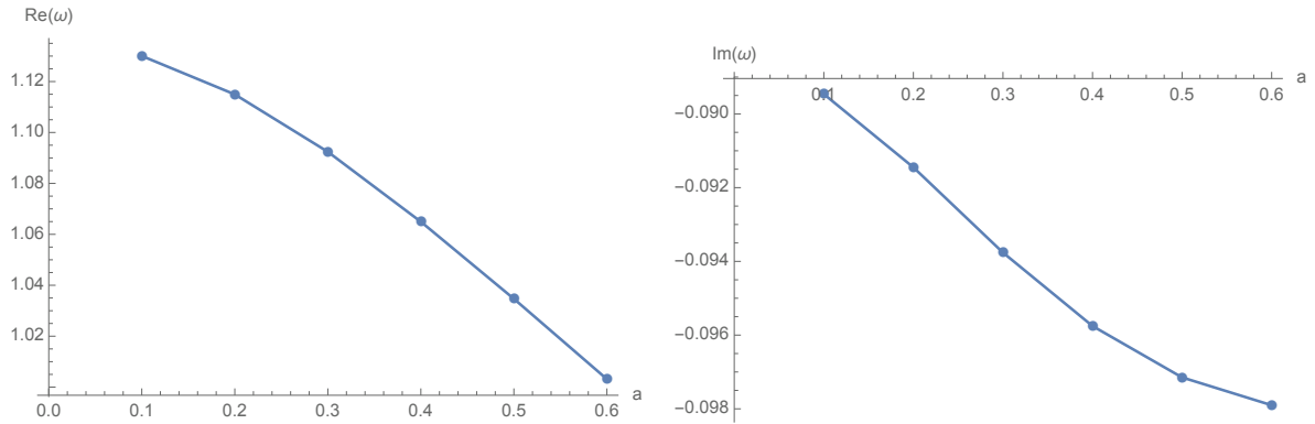
Fig. 5. (color online) The real and imaginary part of QNMs with sixth-order WKB formula for a versus \text{Re}(\omega) and a versus \text{Im}(\omega) for M=1 , s=0 mode with the multipole number l=4 .
